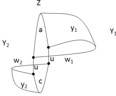
Figure 2: A schematic for the argument that f is surjective.
