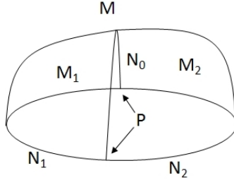
Figure 1: A schematic of the hypothesis of Wall's theorem: The manifold-with-boundary M is split into the pieces M_1 and M_2 along the hypersurface N_0 . The boundary of M is split into N_1 and N_2 along P .
