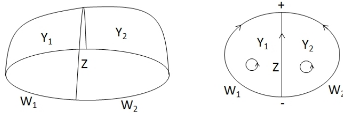
Figure 4: A schematic of a splitting of a \partial -stratified pseudomanifold (left) and a flatter schematic of the relative orientations (right).
