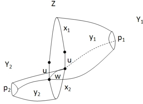
Figure 3: A schematic for the argument that \ker(f) \subset S .
